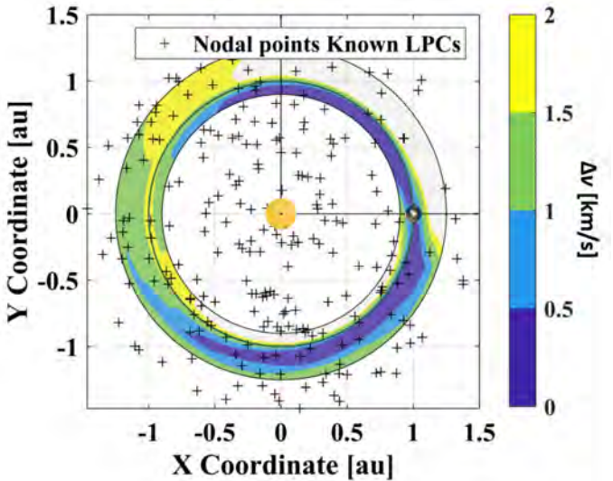
Accessible regions in the ecliptic plane as a function of different spacecraft’s \Delta v capabilities. Credit (image and caption): Cuartielles et al Figure 4.
