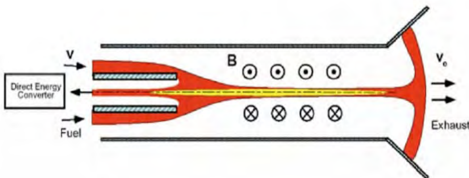
Simple Z-pinch thruster design by Shumlak. The cylindrical magnetic field is towards (above the plasma) and away (below) from you.
